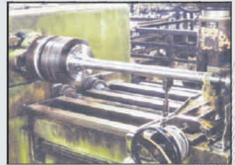
Spline Hobbing
