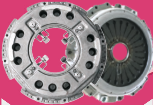
Conventional Cover Assembly
